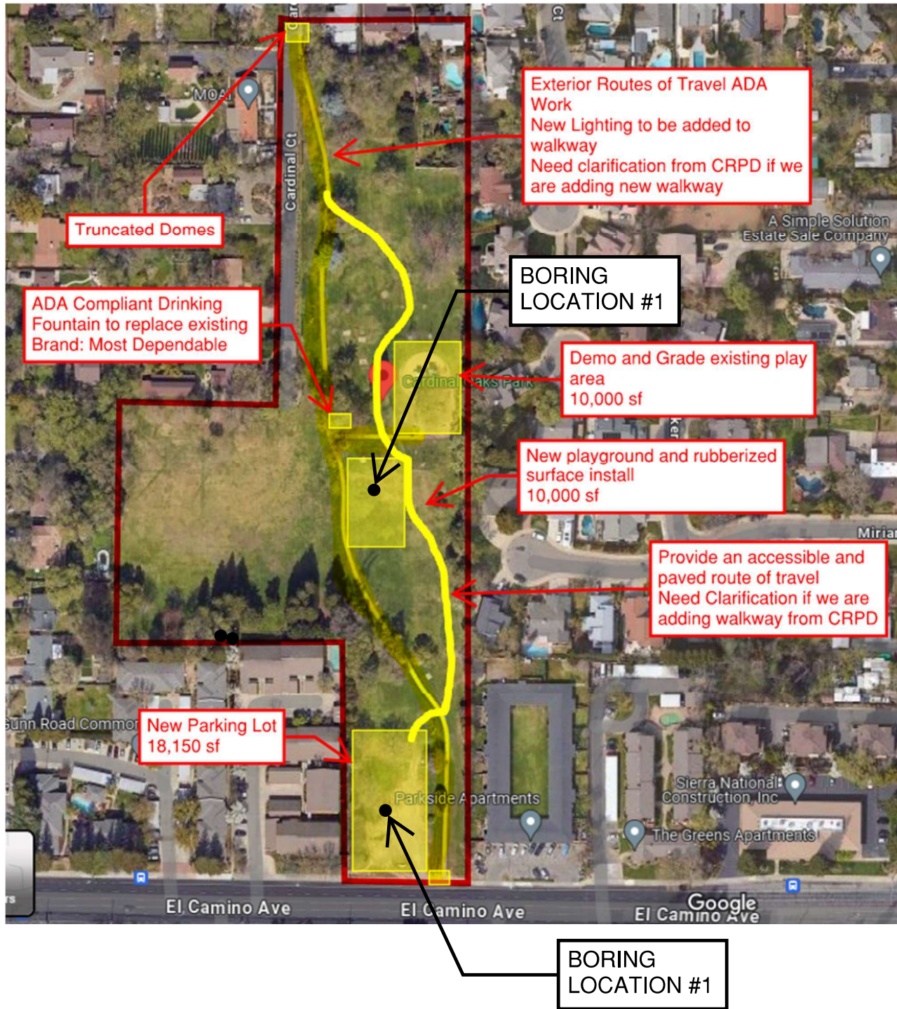
Cardinal Oaks Park Site Plan
